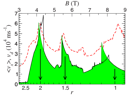
FIG. 10. (Color online) \langle v_x \rangle calculated as a function of increasing (black curve) and decreasing (curve with green shading) B (upper axis). Lower axis shows values of r \propto 1/B . Peaks in \langle v_x \rangle originate from r=1, 3/2 , and 2 resonances (located by arrows). The difference between the two curves originates from the hysteretic evolution of the electron limit cycle discussed in Sec. IV. Dashed curve shows v_d (with no vertical offset) calculated as a function of B (or r ) using Eq. (10). F=10^6 V m ^{-1} , \theta=45^\circ , \alpha=10^{12} s ^{-1} .
