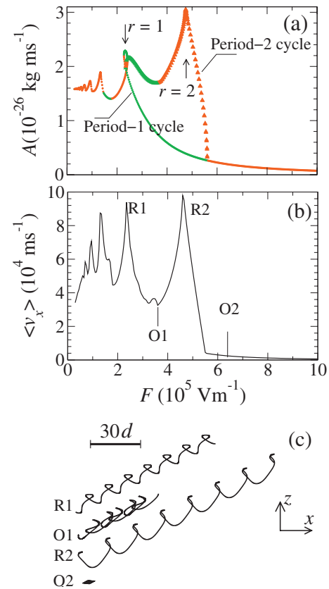
FIG. 8. (Color) (a) Amplitude A of p_z(t) oscillations calculated versus F for a stable (unstable) period-1 limit cycle [red (green) circles] and a stable (unstable) period-2 limit cycle [red (green) triangles]. Arrows mark positions of r=1 and 2 resonances. (b) \langle v_x \rangle calculated as a function of F for the attractor approached by electrons starting from rest. Peaks labeled R1 (R2) occur at F values near the r=1 (2) nonlinear resonances. Labels O1 (O2) mark off-resonance field values for which r=1.52 (2.53). (c) Orbits approached by electrons starting from rest at the resonant (R1,R2) and off-resonant (O1,O2) F values marked in (b). All attractors are projected onto the x - z plane (axes inset), have a common spatial scale shown by the horizontal line whose length is 30 SL periods, and are plotted over the same time interval. B=2 T, \theta=45^\circ , \alpha=10^{12} s ^{-1} .
