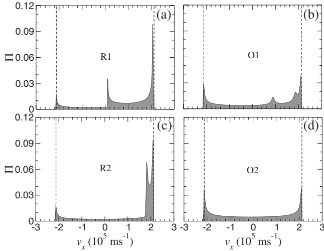
FIG. 9. Normalized \Pi(v_x) curves (with gray shading underneath) calculated for electron trajectories labeled in Figs. 8(b) and 8(c) as (a) R1, (b) O1, (c) R2, and (d) O2. Vertical dashed lines mark extremal velocities v_x = \pm v_{\max} , B=2 T, \theta=45^\circ , \alpha=10^{12} s ^{-1} .
