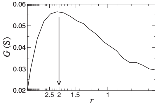
FIG. 11. Experimental values of the low-temperature (4.2 K) differential conductance G=dI/dV versus r=\omega_B/\bar{\omega}_c \propto F/B , measured for different values of B at fixed V=0.25 V and \theta=45^\circ for the SL described in Ref. [15], whose parameters are similar to those specified in Sec. II. Arrow marks r=2 resonance.
