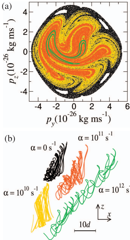
FIG. 3. (Color) (a) Black dots: stroboscopic Poincaré section calculated for an electron trajectory starting from rest in the dissipationless limit \alpha=0 . Colored dots: stroboscopic Poincaré sections calculated for the chaotic attractors of electrons starting from rest when \alpha=10^{10} (yellow dots), 10^{11} (red dots), and 10^{12} \text{ s}^{-1} (green dots). (b) Electron trajectories corresponding, by specified value of \alpha and color, to the Poincaré sections shown in (a). All orbits are projected onto the x - z plane (axes inset), have a common spatial scale shown by the horizontal line whose length is 10 SL periods, and are plotted over a fixed time interval of 22.68 ps, which is long enough to reveal the form of the electron trajectories. B=4.75 \text{ T} , \theta=45^\circ , F=7.5 \times 10^5 \text{ V m}^{-1} , r \approx 1.33 .
