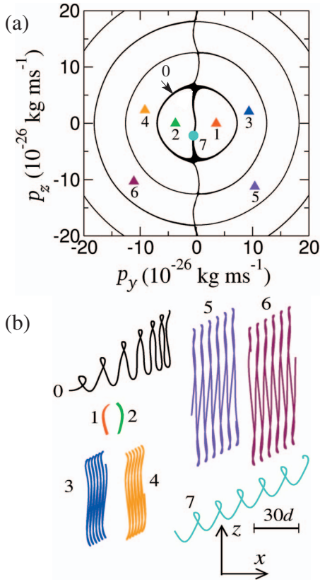
FIG. 2. (Color) (a) Black dots: stroboscopic Poincaré section calculated for the chaotic trajectory executed by an electron starting from rest in the dissipationless limit \alpha=0 . This section reveals the inner filaments of a stochastic web. Colored triangles numbered 1–6: Poincaré sections calculated for six coexisting stable limit cycles formed when \alpha=10^{10} \text{ s}^{-1} . Blue circle numbered 7: Poincaré section calculated for the single stable limit cycle found when \alpha=10^{12} \text{ s}^{-1} . (b) Electron trajectories corresponding, by number and color, to the labeled features in the Poincaré sections shown in (a). All orbits are projected onto the x - z plane (axes inset), have a common spatial scale shown by the horizontal line whose length is 30 SL periods, and are plotted over a fixed time interval of 9.45 ps. The field parameters B=2 \text{ T} , \theta=30^\circ , and F=2.9 \times 10^5 \text{ V m}^{-1} satisfy the resonance condition \omega_B/\bar{\omega}_c=1 .
