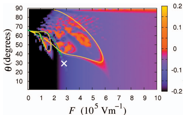
FIG. 7. (Color) (a) Color map showing \lambda calculated as a function of F and \theta for the attractors approached by electron trajectories starting from rest when B=2 T and \alpha=10^{12} s ^{-1} . Color scale is shown on the right. Yellow (green) curves are loci of period-doubling (saddle-node) bifurcations of electron limit cycles. Cross marks (F, \theta) coordinate corresponding to limit cycle 7 in Fig. 2.
