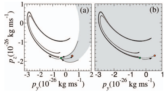
FIG. 6. (Color) Stroboscopic Poincaré sections calculated at times t=lT_B ( l=0, 1, 2, \dots ) when B \approx (a) 2.46 T just before boundary crisis, (b) 2.461 T at the boundary crisis. The sections are constructed by plotting (p_y, p_z) whenever \dot{p}_z=0 along the chaotic attractor for electrons starting from rest (black dots), and for the stable period-1 limit cycle (red circles) and unstable saddle period-1 limit cycle (green circles), which are formed by saddle-node bifurcation SN1 in Fig. 5. White (gray) regions are basins of attraction for the chaotic attractor and stable period-1 limit cycle respectively. Arrows in (a) pointing toward (away from) the green circle represent stable (unstable) manifolds of the unstable saddle period-1 limit cycle. Arrow and dotted curve in (b) show the direction along which the electron trajectory eventually leaves the chaotic attractor and subsequently approaches the stable period-1 limit cycle. F=3 \times 10^5 V m ^{-1} , \theta=45^\circ , and \alpha=10^{12} s ^{-1} .
