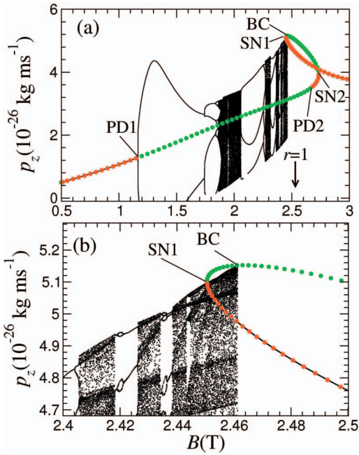
FIG. 5. (Color) (a) Poincaré sections constructed by plotting p_z whenever \dot{p}_z=0 along limit cycles for electrons starting from rest (black dots) and for stable (unstable) period-1 limit cycles [red (green) circles] with F=3 \times 10^5 V m ^{-1} , \theta=45^\circ , and \alpha=10^{12} s ^{-1} . Increasing B induces period-doubling (PD1, PD2) and saddle-node (SN1, SN2) bifurcations, which correspond to crossing the black and green curves along the blue arrow in Fig. 4(c), and a boundary crisis (BC). Arrow marks B value for which r=1 . (b) An enlargement of the Poincaré section in the vicinity of saddle-node bifurcation SN1 and boundary crisis BC.
